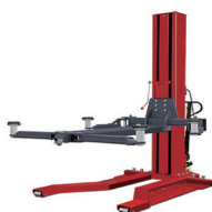
SINGLE POST LIFT Mobile post or fixed post Capacity: 2.5T
